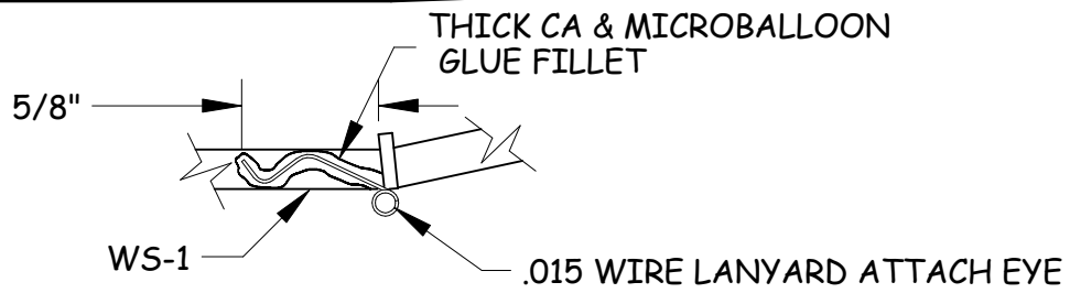
VIEW XA-XA
